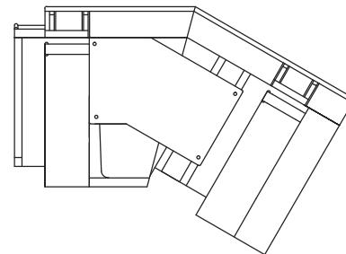
SIZE 250 - Gradient Trough (down) (GT-250-06)
